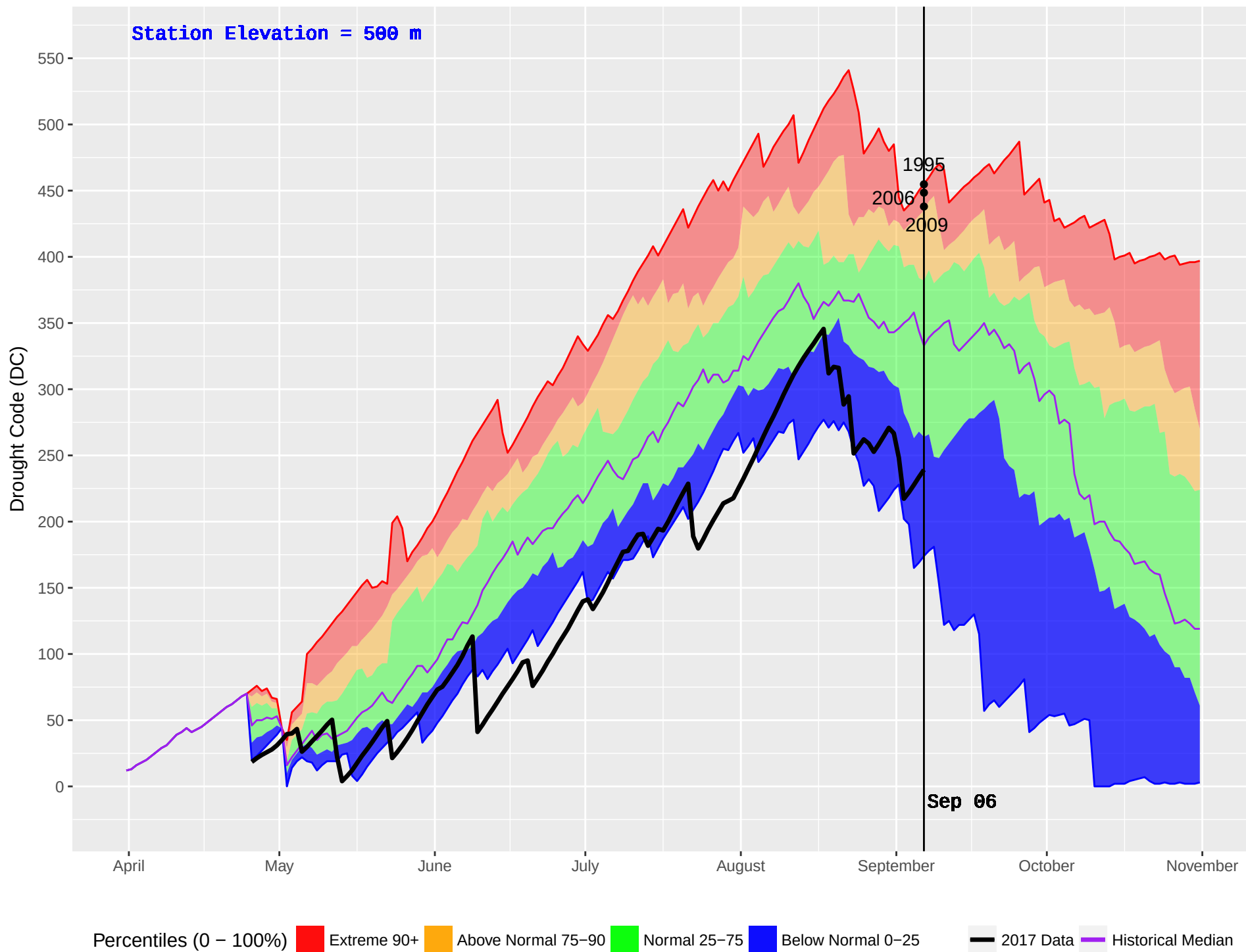
CRANBERRY (433) : Historical (1995–2016) and Current (2017) Noon Drought Code (DC)
