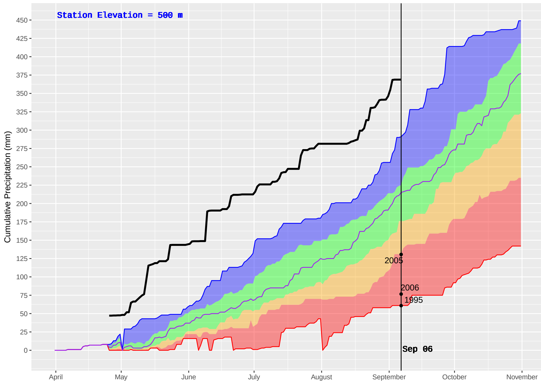
CRANBERRY (433) : Historical (1995–2016) and Current (2017) Noon Cumulative Precipitation
